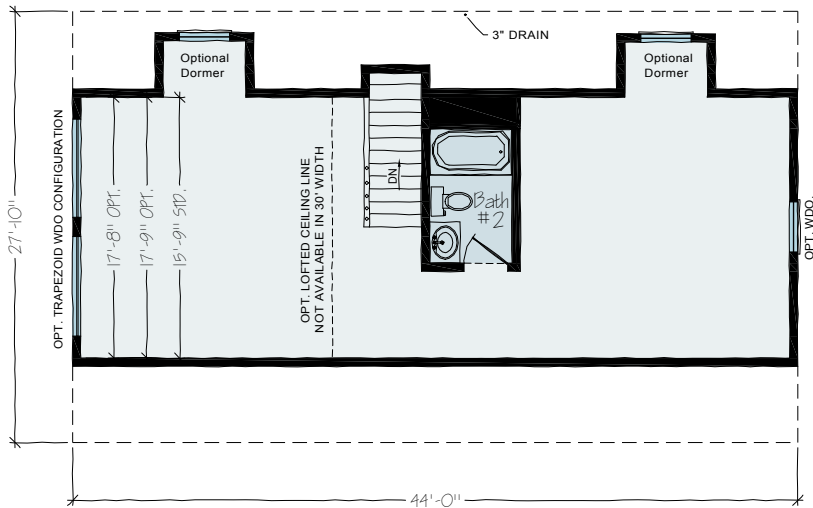
PURPOSED SECOND FLOOR LAYOUT (FINISHED ON SITE BY OTHERS.)
