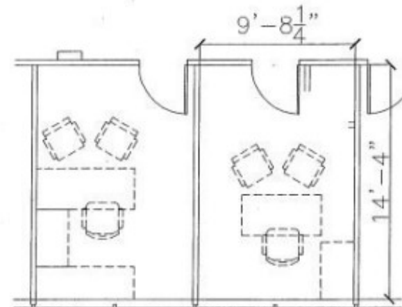
① TYPICAL OFFICE LAYOUTS SCALE: 1/8"=1'-0"
