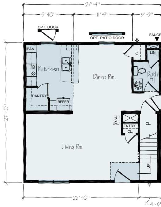
TS 14 1ST FLOOR
