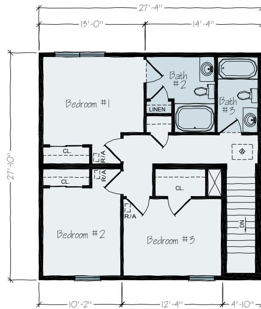
TS14 2ND FLOOR
