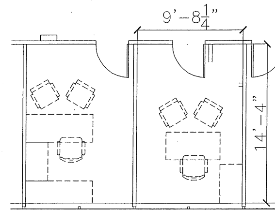
① TYPICAL OFFICE LAYOUTS SCALE: 1/8"=1'-0"
