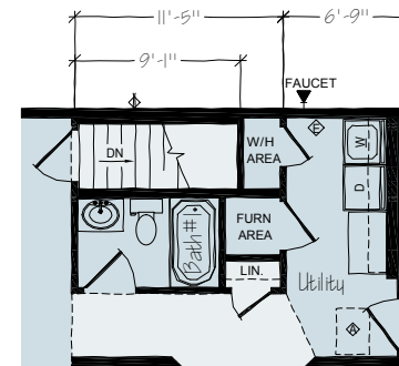
OPT. STAIRWAY LAYOUT
