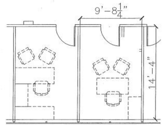
① TYPICAL OFFICE LAYOUTS SCALE: 1/8"=1'-0"
