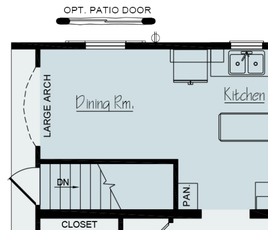
BASEMENT OPTION
