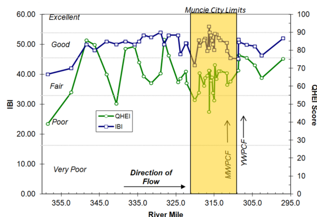
Figure 5.—Average IBI and QHEI scores from WFWR (2004-2016).
