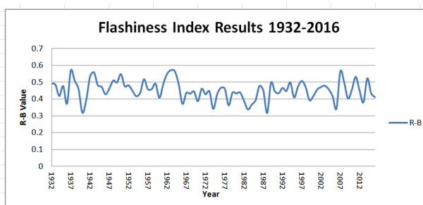
Figure 3.— Richard-Baker Flashiness Index Results 1932-2016.
