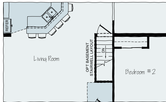
OPT. STAIRWAY LAYOUT
