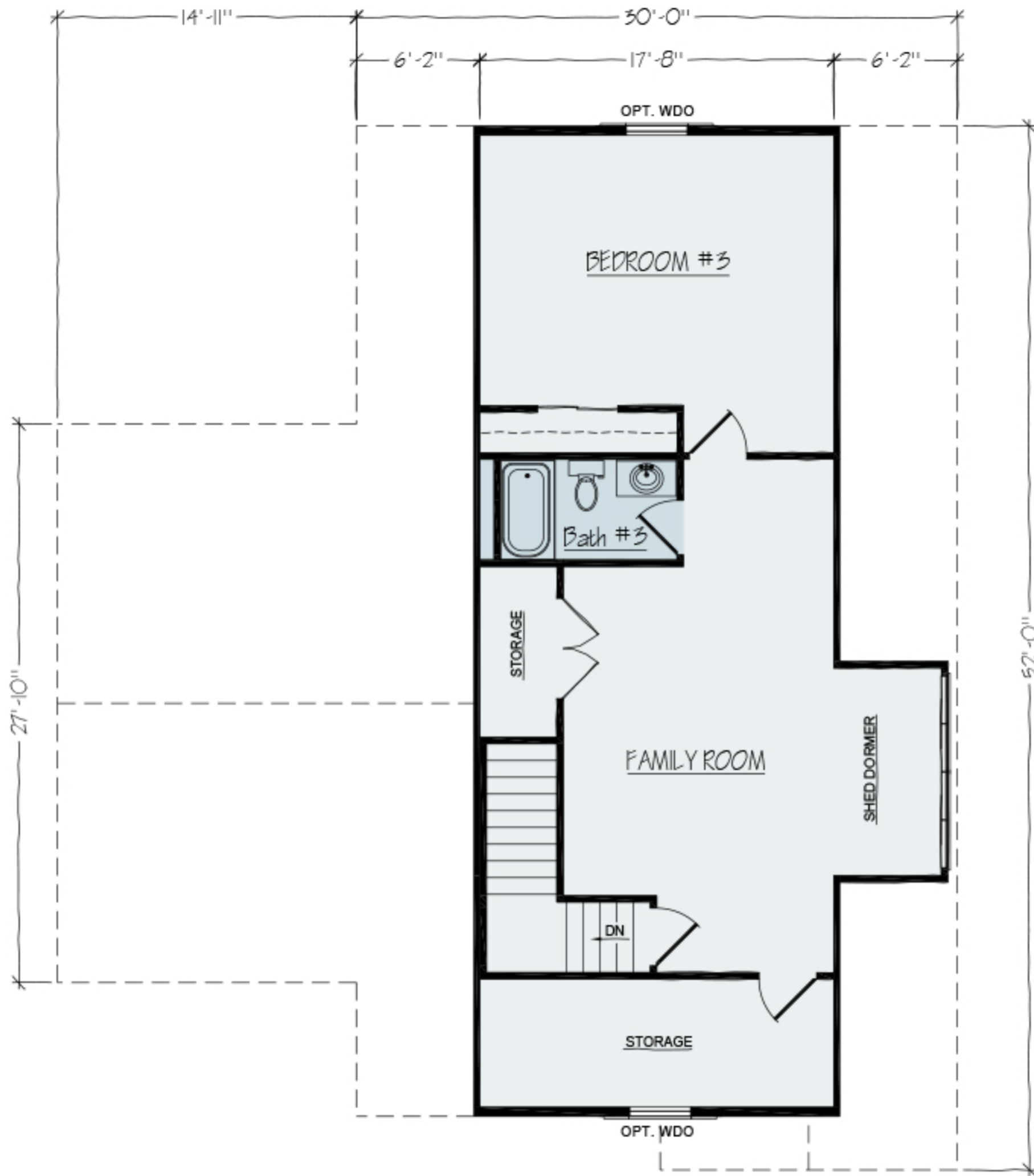
OPTIONAL SECOND FLOOR LAYOUT
