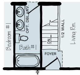
OPT. BASEMENT STAIRWELL LAYOUT
