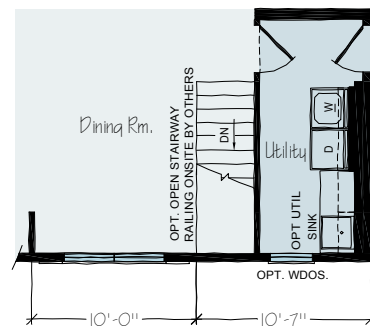
OPT. BASEMENT STAIRS
