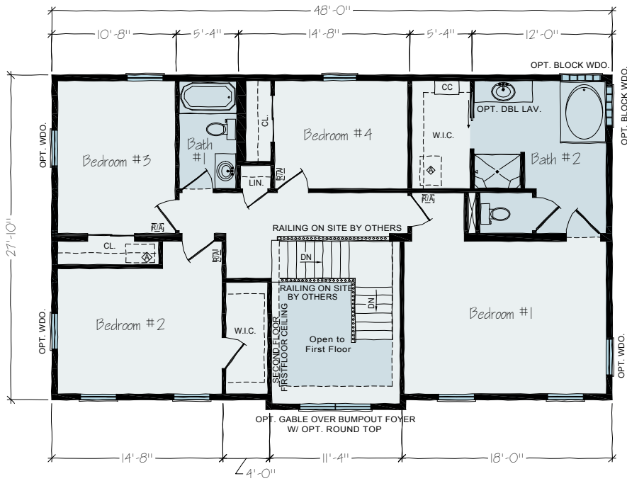
2ND FLOOR
